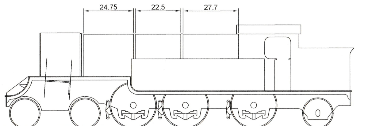
Boilerband Dimensions.
